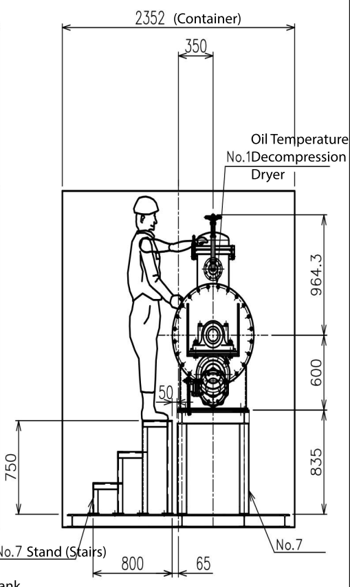
Oil Temperature No.1 Decompression Dryer B-B Arrow View
