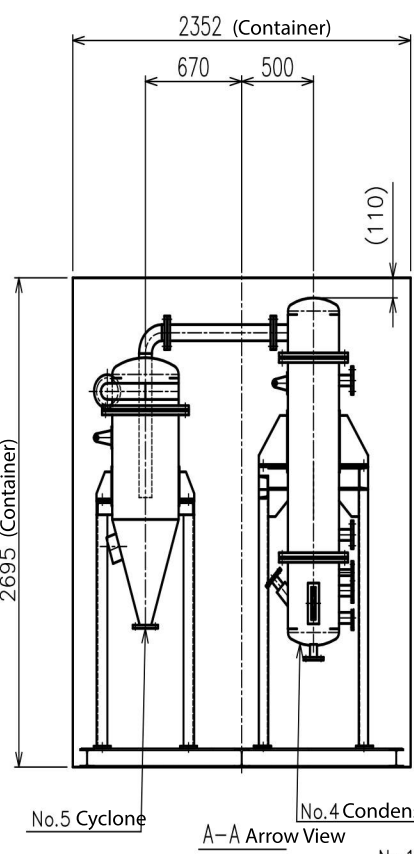
No.5 Cyclone A-A Arrow View
