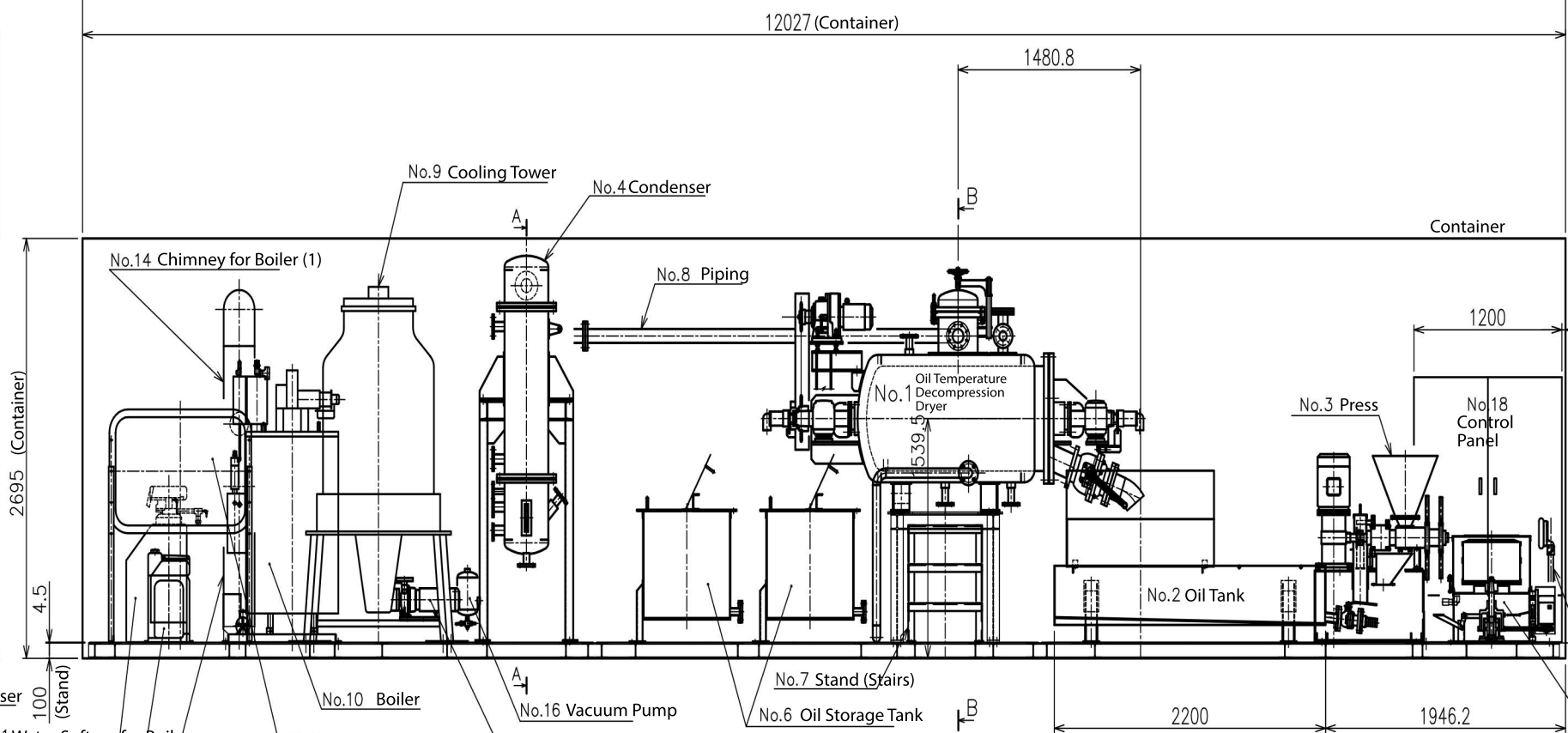
No.11 Water Softner for Boiler No.13 Chemical Injection Systems for Boiler No.14 Chimney for Boiler (1) No.10 Boiler No.16 Vacuum Pump No.17 Water Supply Pump No.8 Piping No.4 Condenser No.6 Oil Storage Tank No.7 Stand (Stairs) No.1 Oil Temperature Decompression Dryer No.2 Oil Tank No.3 Press No.18 Control Panel
